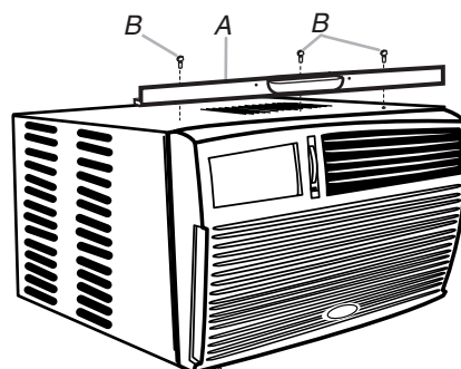
A. Top channel B. #10 x \frac{3}{8} " pan-head screw
