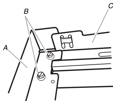
A. Tray back B. #8 - 18 x \frac{1}{4} " hex-head screws C. Tray side
